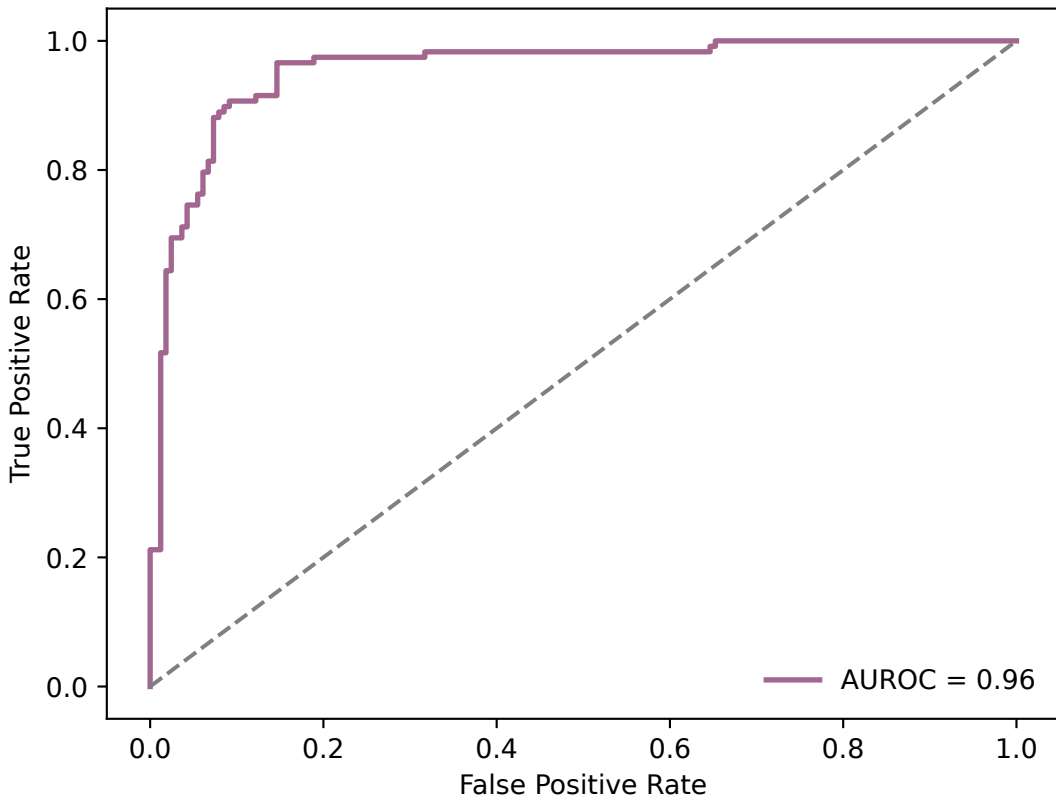
LOGISTIC ROC Curve
